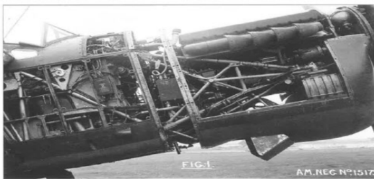
The starboard side of one of the prototype Barracuda MB.V aircraft with cowling panels over its Rolls Royce Griffon engine removed. The extra 'bay' fitted to the nose to accommodate the longer engine can be discerned. The exhaust manifold with four fishtail stubs is visible. (National Archives)
