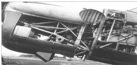
The port side of the same aircraft. On this side, the large 'trumpet' shroud for the exhaust, intended to provide sufficient cooling with flame damping for night-flying, is still fitted. The large semi-circular board radiator required by the Griffon can be seen in the lower-forward portion of the cowling. (National Archives)
